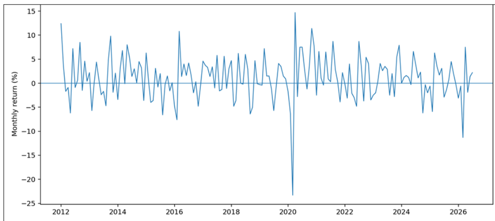
Fig 1: NIFTY 50 monthly price returns (%), January 2012–July 2026 [28] .
