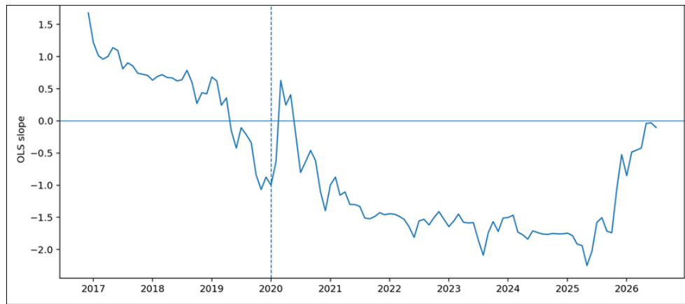
Fig 5: Rolling 60-month OLS slope of NIFTY 50 returns on the 10-year yield. The dashed vertical line marks January 2020.
