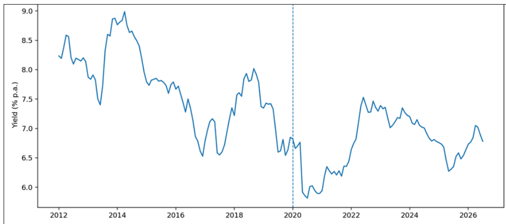
Fig 2: India 10-year government-security yield (% p.a.), January 2012–July 2026 [28] .
