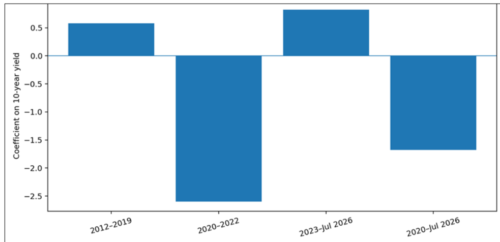
Fig 4: Regime-specific coefficients on the 10-year yield.
