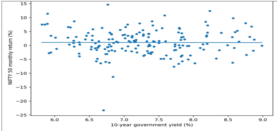
Fig 3: NIFTY 50 monthly returns (%) against the 10-year yield (%) with fitted baseline regression line.
